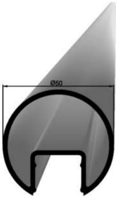
GLASS COVER PROFILE Ø50X2 2919
