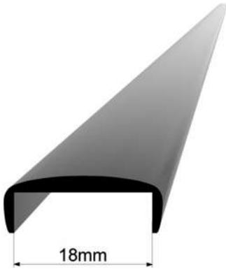
GLASS COVER PROFILE 6023
